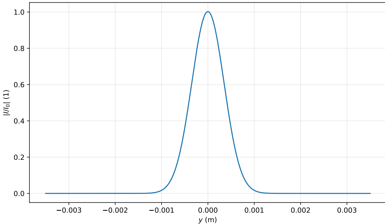
Intensity profile I(x=0, y, z=0.080)/I_0 , \text{Pin}=0.6\text{Pcr} , artificial time
